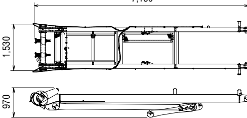
Gantry Weight: 2,950 kg
