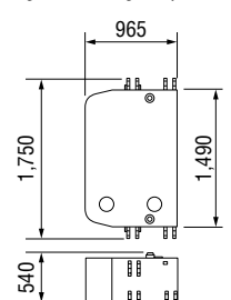
Carbody Weight B Weight: 5,000 kg x 2 pieces
