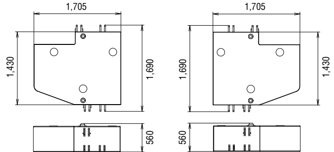
Counterweight No.2 Weight: 5,000 kg / 1 piece
