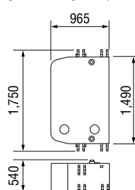
Counterweight B Weight: 5,000 kg x 10 pieces
