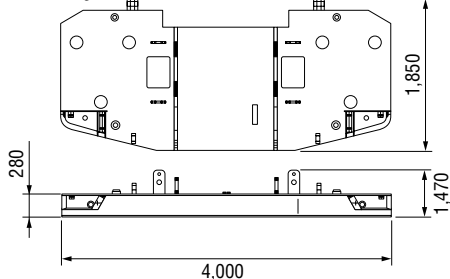
Counterweight A Weight: 10,000 kg
