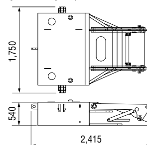
Carbody Weight A Weight: 5,000 kg x 2 pieces
