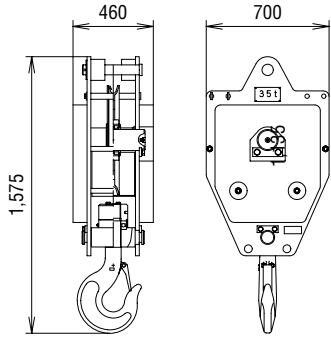
35 t Hook Block Weight: 900 kg
