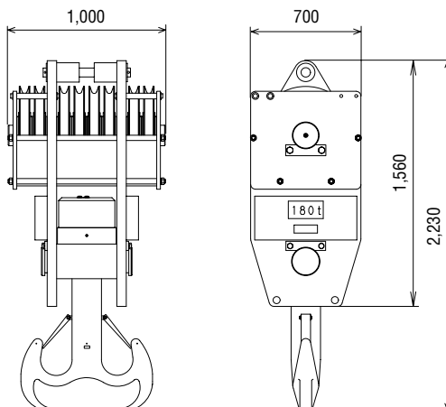
180 t Hook Block Weight: 2,800 kg
