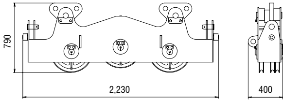
Luffing Boom Tip Assembly Weight: 6,600 kg
