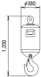
Ball Hook Weight: 460 kg
