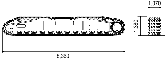
Crawler Weight: 17,200 kg
