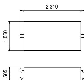
Carbody Weight No.2 Weight: 5,000 kg / 1 piece
