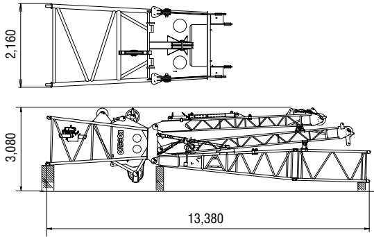
Luffing Boom Tip Assembly Weight: 6,600 kg
