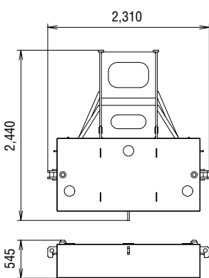
Carbody Weight No.1 Weight: 5,065 kg / 1 piece
