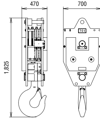
70 t Hook Block Weight: 1,200 kg
