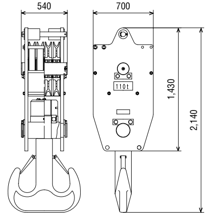
110 t Hook Block Weight: 1,730 kg
