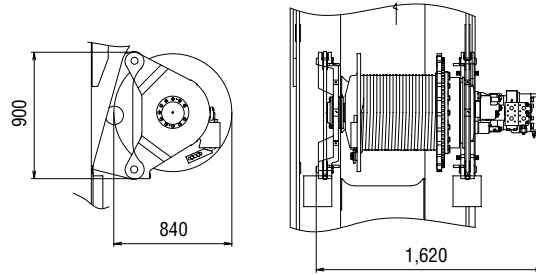
Luffing Jib Drum Weight: 1,470 kg
