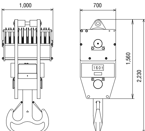
160 t Hook Block Weight: 2,800 kg
