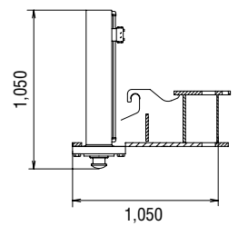
Translifter Weight: 360 kg
