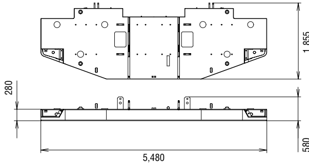
Carbody Weight No.1 Weight: 5,065 kg / 1 piece
