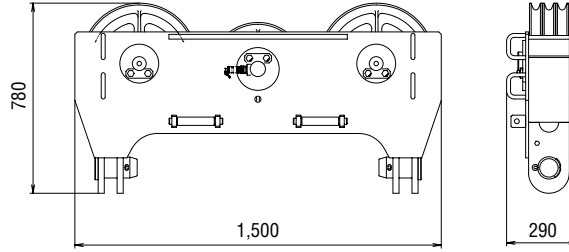
Luffing Jib Drum Weight: 1,470 kg
