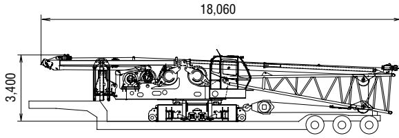
Base Machine Weight: 43,450 kg
